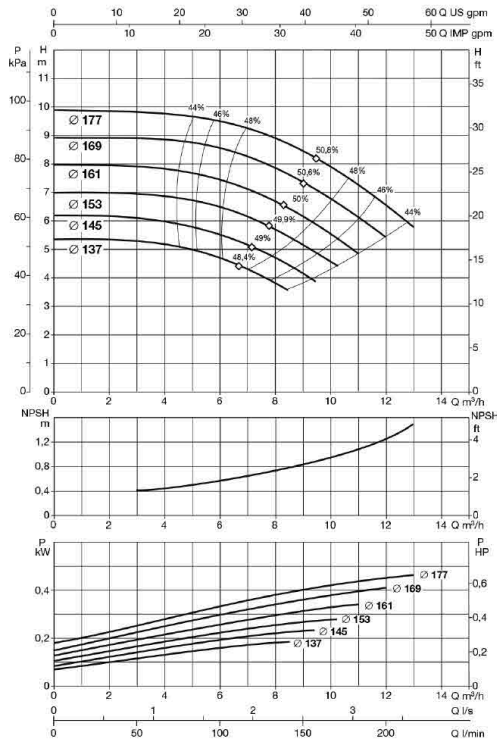
KDN 32-160.1
